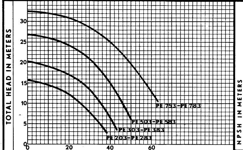
IMPELLER NO. * FLOW - M 3 /hr. Curve 4848292
