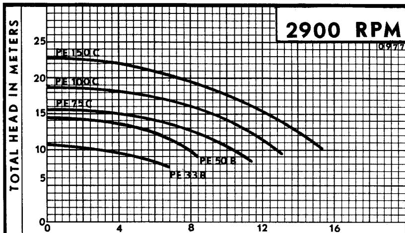
IMPELLER NO. * FLOW - M 3 /hr. Curve 4848291
