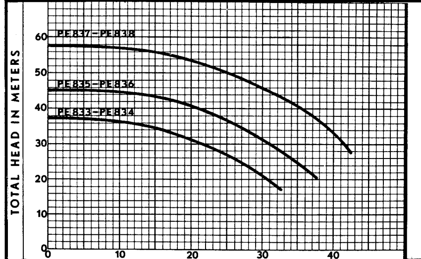
IMPELLER NO. * FLOW - M 3 /hr. Curve 4848293
